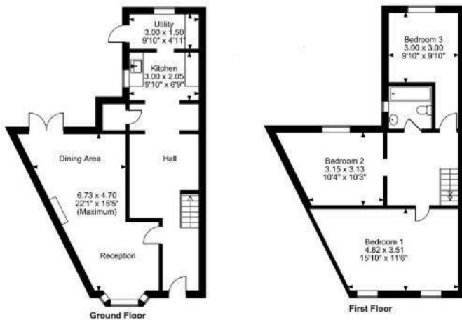
Evesham Road Approximate Gross Internal Area Main House = 1257 Sq Ft/117 Sq M
